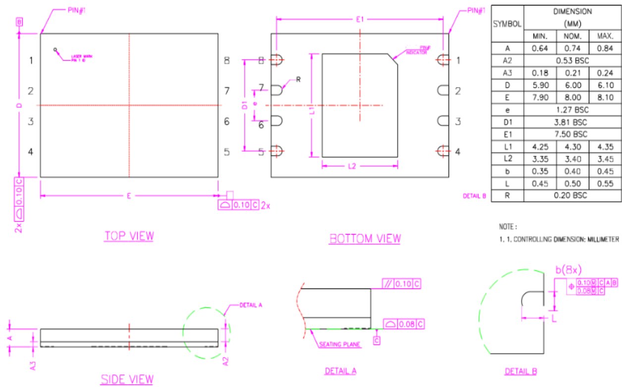
Figure 6.2 LGA (8*6mm)
