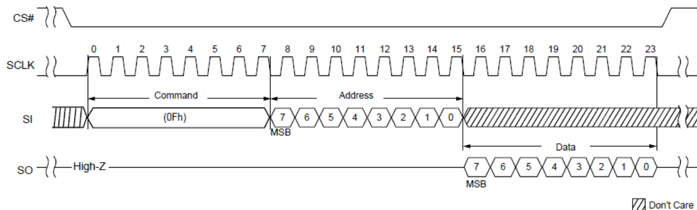
Figure 3.3 Get Features(0Fh)
