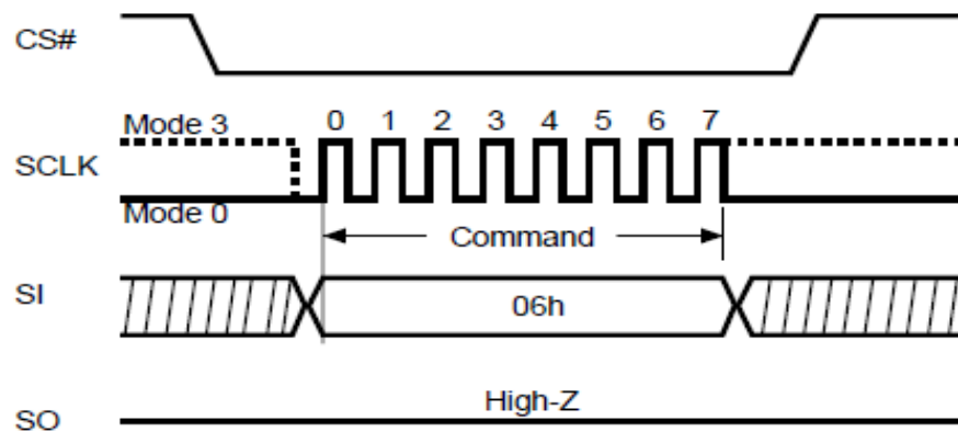
Figure 3.1 Write Enable
